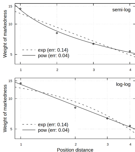
Figure 4. Exponential (dashed, ‘exp’) and power law (solid, ‘pow’) fits to English liquid dissimilation data. Data points are shown as open circles. Regression errors (‘err’) are in parentheses.
