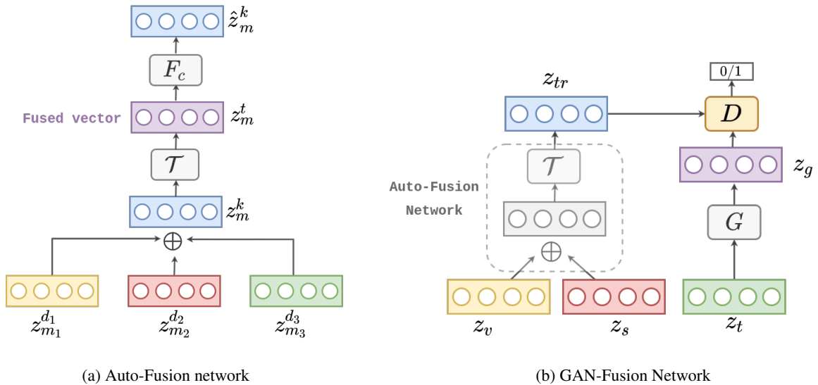
Figure 1: Proposed architectures. (a) Auto-Fusion network: Assuming that z_{m_1}^{d_1} , z_{m_2}^{d_2} , and z_{m_3}^{d_3} represent the video, speech, and text latent vectors respectively, we first concatenate them to obtain z_m^k . It is then passed through \mathcal{T} which outputs the “autofused” vector z_m^t . We then obtain the reconstructed concatenated vector \hat{z}_m^k by passing the autofused vector through F_c , another transformation layer. Finally, we optimize the loss between \hat{z}_m^k and z_m^k . (b) GAN-Fusion module for the text modality: Assuming that z_s , z_v , and z_t are the latent speech, video, and text vectors, respectively, we first autofuse z_s and z_v to give z_{tr} . Simultaneously, we pass z_t through the generator G , along with some noise, to get z_g . The generator loss tries to match z_{tr} and z_g and discriminator D tries to distinguish between z_{tr} and z_g , the two sources of input. Note: \oplus denotes concatenation.
