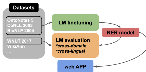
Figure 1: System overview of T-NER.
