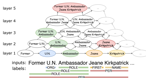
Figure 1: Pyramid output of a sentence from NNE (Ringland et al., 2019) containing 8 nested entities.
