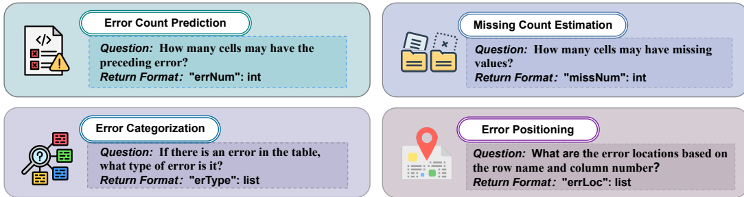
Figure 5: Exemplifying inputs and outputs of four evaluation sub-tasks.
