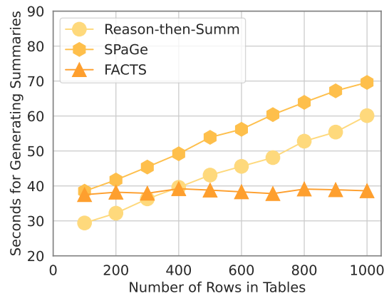
Figure 4: Scalability analysis. Runtime for generating summaries as the number of rows in each table increases.
