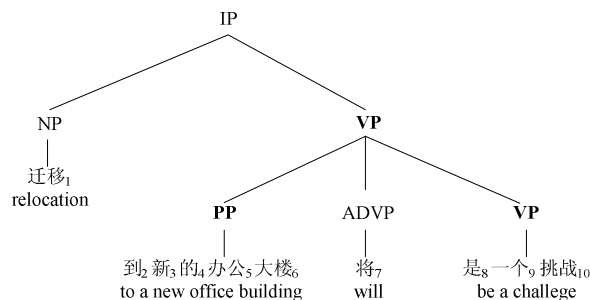
Figure 2: The simplified Chinese parse tree of the example sentence and the leaves are Chinese words with their index and corresponding English translation.
