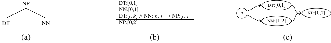
Figure 1: Three views of parsing: (a) tree construction, (b) logical deduction, and (c) hypergraph exploration.
