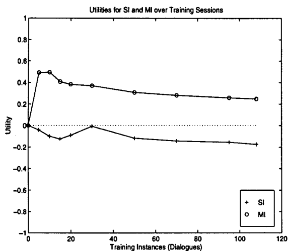
Figure 1: Results of applying Q-learning to System-Initiative (SI) and Mixed-Initiative (MI) Strategies for 108 ELVIS Dialogues
