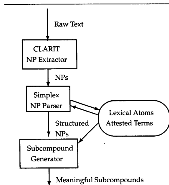
Figure 1: General Processing for Phrase Generation
