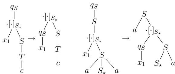
Figure 10: Two constructed XTT rules.
