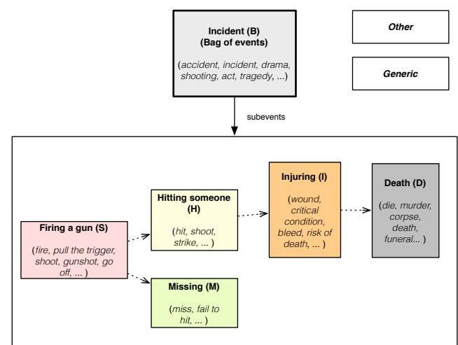
Figure 3: The event scheme used for the annotation of gun violence events.
