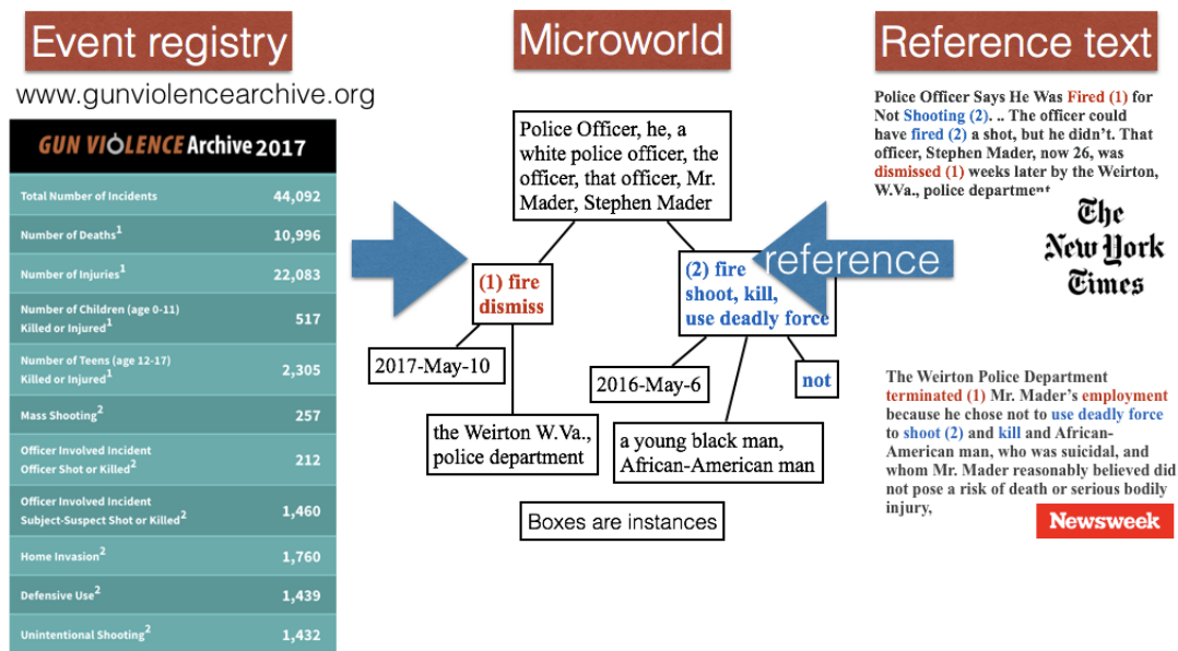
Figure 2: Overview of the D2T method: representing structured event data first as microworlds and secondly pairing it with reference texts.
