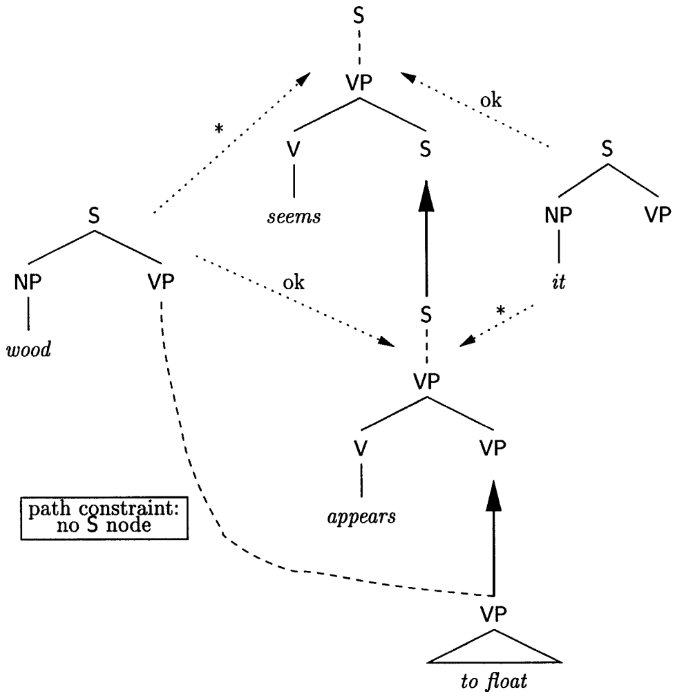
Figure 21 Path constraints are needed to rule out ungrammatical super-raising.
