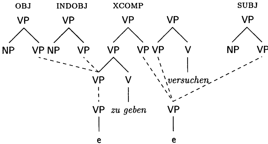
Figure 24 DSG derivation for a complex sentence.
