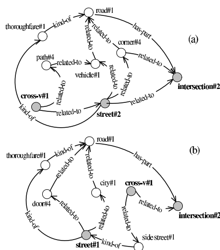
Figure 1: (a) Semantic interconnection patterns supporting the choice of sense #2 of street in sentence (a). (b) Some interconnections supporting the choice of street#1 for the same sentence.
