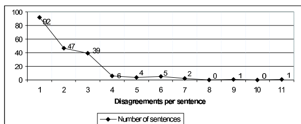
Figure 3: Distribution of the number of disagreements in the subset of the Senseval-3 test set.
