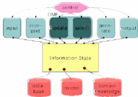
Figure 1: GoDiS architecture
