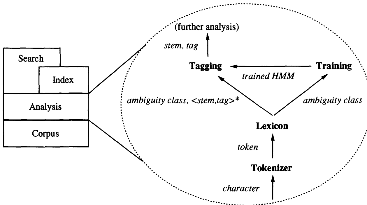
Figure 1: Tagger Modules in System Context
