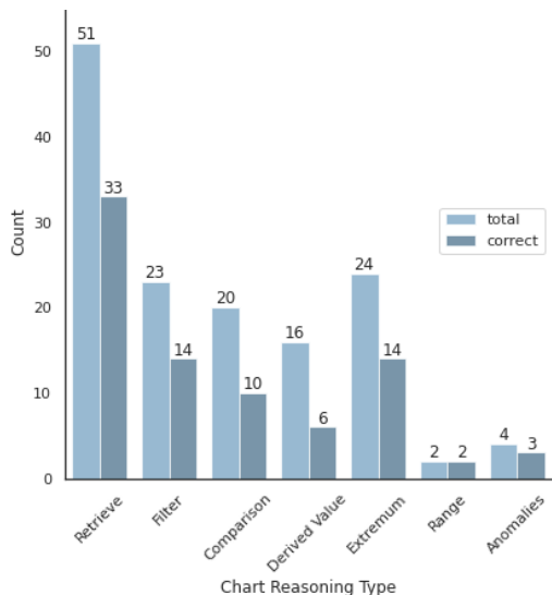
Figure 6: Chart reasoning types: total count and correct predictions of manually annotated test samples.
