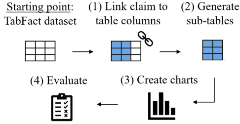
Figure 4: Dataset creation process.
