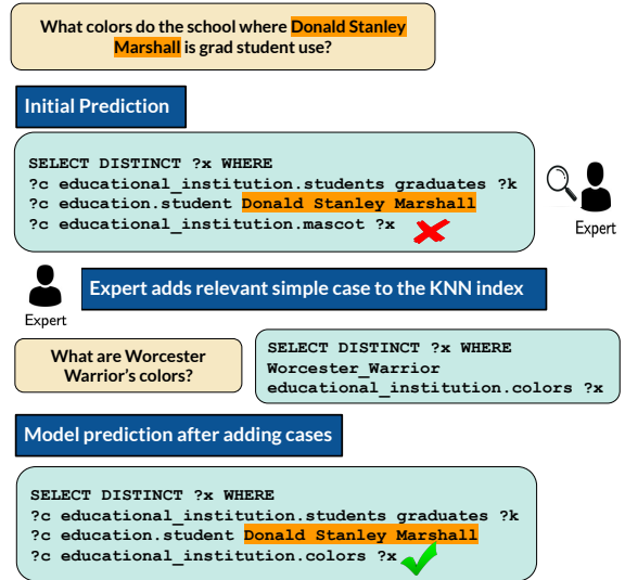
Figure 3: An expert point-fixes a model prediction by adding a simple case to the KNN index. Initial prediction was incorrect as no query with the relation (educational_institution.colors) was present in the train set. CBR-KBQA retrieves the case from the KNN index and fixes the erroneous prediction without requiring any re-training.
