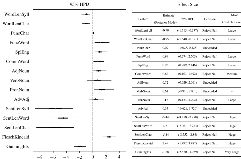
Figure 6: 95% HPD and the most credible levels for effect sizes ( \frac{\mu_{\text{online}} - \mu_{\text{offline}}}{\sqrt{(\eta^2_{\text{online}} + \eta^2_{\text{offline}})/2}} ). The ROPEs are set with (-0.1, 0.1) associated with Cohen’s “small” effect ( d=0.2 ).
