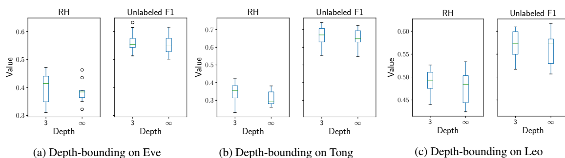
Figure 5: Comparison of labeled and unlabeled evaluation of grammars bounded at depth 3 and unbounded grammars on English (Eve), Chinese Mandarin (Tong) and German (Leo) datasets from CHILDES.
