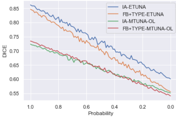
Figure 2: Change of the performance with respected to different probabilities of inserting superfluous TYPE for either the FB+TYPE and IA on either the people domain of MTUNA-OL and ETUNA.
