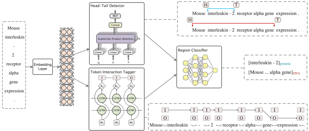
Figure 2: An overview of the proposed HIT model.
