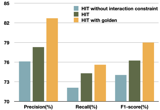
Figure 3: Results on HIT of different structures.
