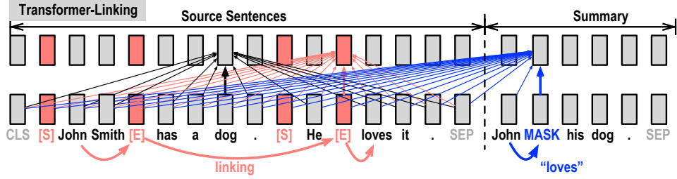
Figure 2: Our TRANS-LINKING model facilitates summary generation by reducing the shifting distance, allowing the model attention to shift from “John” to the tokens “[E]” then to “loves” for predicting the next summary word.
