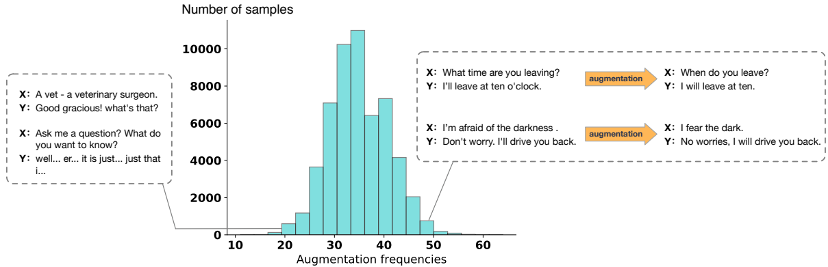
Figure 5: Examples with different augmentation frequencies. Instances with higher augmentation frequencies are more effective than those seldom augmented examples.
