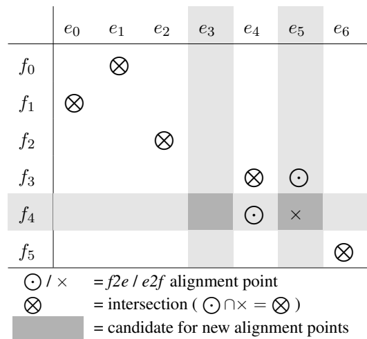
Figure 1: Choosing the candidates for the word pairing and the candidate positions for the new intersecting alignment points.
