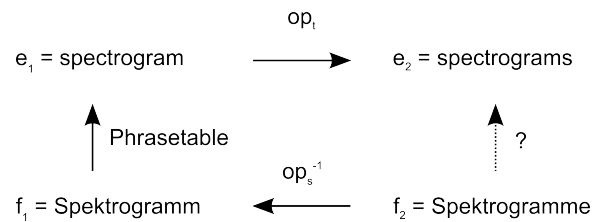
Figure 1: Quasi-morphological operations
