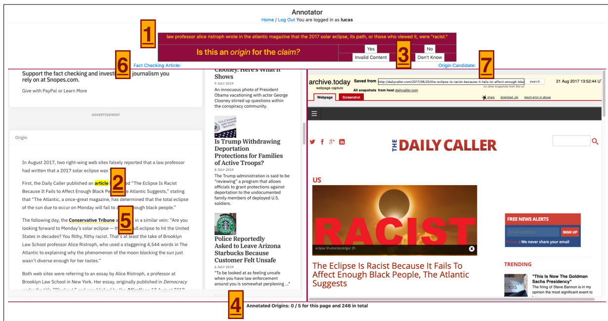
Figure 1: Annotator Interface
