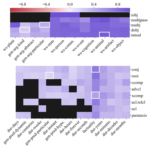
Figure 12: \rho on argument (top) and predicate (bottom) UDS properties (subset) at relevant UD relations. Black cells indicate no significant correlation. Outlined boxes plotted in detail in Figure 11.
