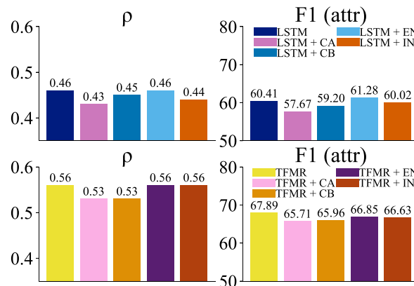
Figure 5: LSTM and TFMR attribute \rho and binarized F1 score.
