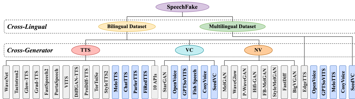
Figure 2: Overview of the SpeechFake dataset. The dataset is divided into two parts: the Bilingual Dataset and the Multilingual Dataset. The Bilingual Dataset is further categorized into three generation methods: TTS, VC, and NV. Methods highlighted in blue represent the latest speech generation methods.
