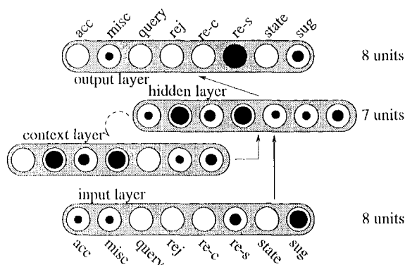
Figure 2: Dialog act network with dialog plausibility vectors as input
