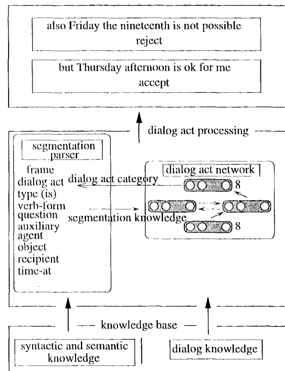
Figure 1: Architecture of dialog act component
