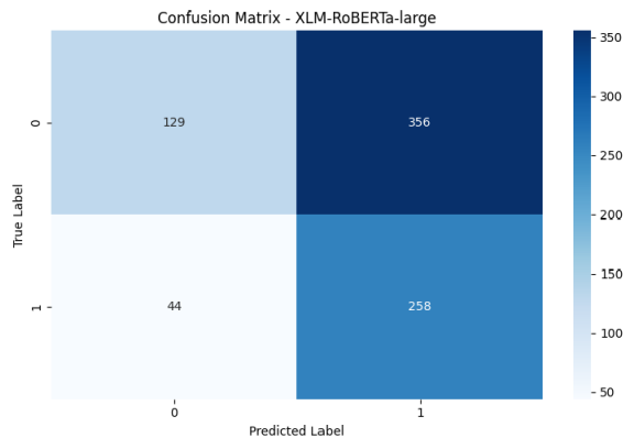
Figure 1: Confusion Matrix
