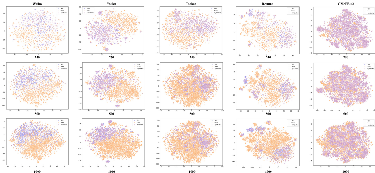
Figure 5: t-SNE visualization of the training, test and enriched explanation samples under different sampling sizes. The synthetic enriched explanation samples are generated by ChatGLM3-6B, and they are represented by the “Synthetic” in the legend.
