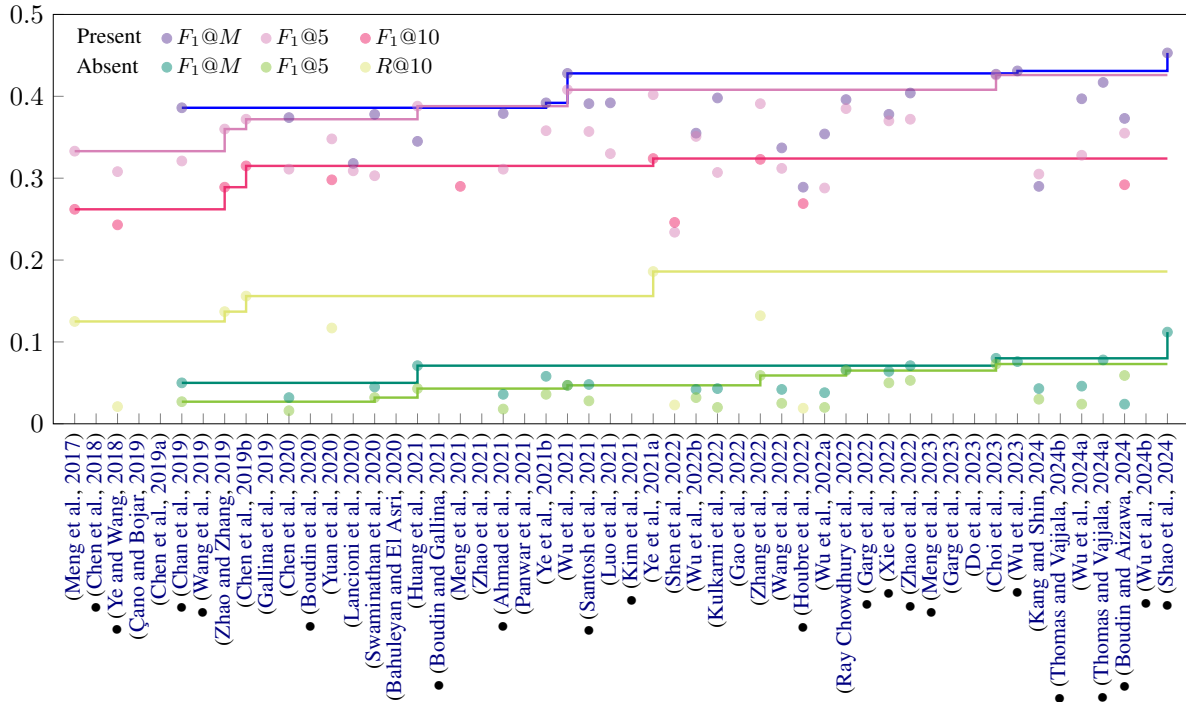
Figure 6: Best scores achieved by each model in terms of F_1@M , F_1@5 and F_1@10 for present keyphrases and F_1@M , F_1@5 and R@10 for absent keyphrases on the KP20k dataset. The lines represent the state-of-the-art performance over time. • indicate that the paper utilizes statistical tests to validate the significance of the results.
