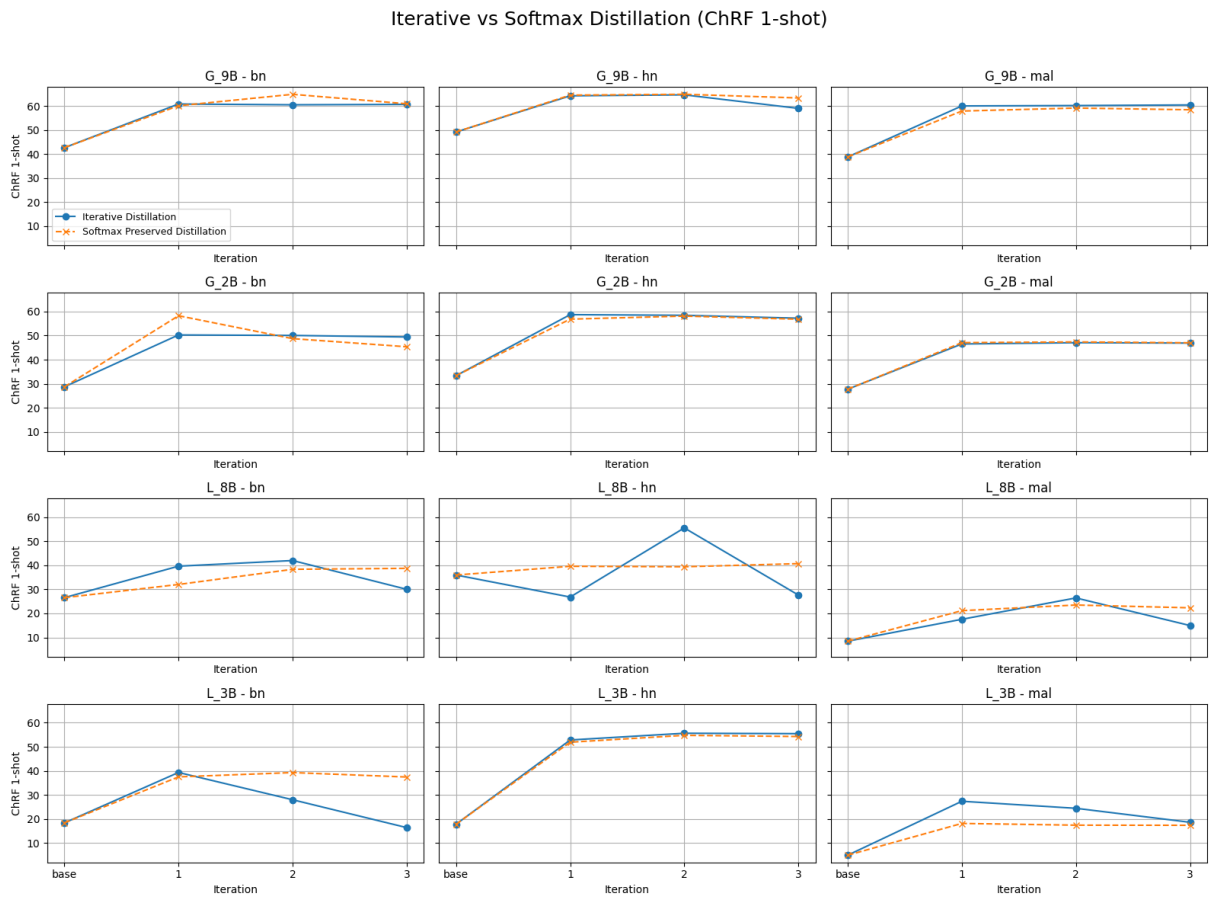
Figure 8: Comparison of methods in the 1-shot setting.
