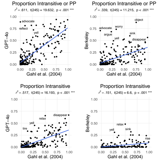
Figure 5: Evaluating the effect of including PP frames in intransitivity counts. For both the GPT-4o (left) and Berkeley (right) parsers, including PPs (as Gahl et al. (2004) did) produced a better fit (top) to Gahl et al.’s estimates than excluding them (bottom), meaning that Gahl et al. lost meaningful information by collapsing these categories.
