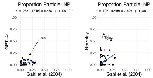
Figure 10: Comparing our estimates of particle-NP (e.g., pick [up] part. [your clothes] NP ) frequencies per verb to Gahl et al. (2004). GPT-4o (left) accounted for more variance than the Berkeley Neural Parser (right).
