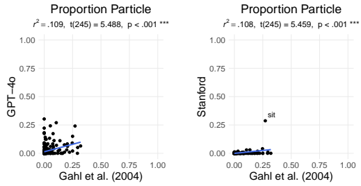
Figure 16: Comparing our estimates of particle (e.g., clean up ) frequencies per verb to Gahl et al. (2004). GPT-4o (left) accounted for the same amount of variance as the Stanford Parser (right), although whatever success the Stanford model had here was largely driven by one verb: sit .
