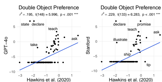
Figure 22: Evaluating the GPT-4o (left) and Stanford (right) Parsers’ estimates of DO/PD bias for dative verbs. We compared estimates to Hawkins et al.’s (2020) relative preference ratings. Many of the verbs they included are non-alternating (e.g., whisper ), and for the majority of these neither GPT-4o nor the Stanford parser identified any DO completions. To avoid infinities, we set proportions of 0 (no instances) or 1 to .001 and .999, respectively, capping log-odds values at \pm 6.907 (the row of black dots at the bottom of each plot). Both parsers significantly predicted preference ratings, accounting for comparable amounts of variance (GPT-4o r^2 = .195 ; Stanford r^2 = .229 ), although Bayesian model comparison revealed “decisive” evidence in favor of the GPT-4o estimates.
