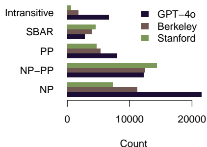
Figure 1: Counts of the five most frequent verb frames (out of 61,427 sentences), by parser.
