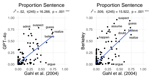
Figure 8: Comparing our estimates of sentential complement (SC; e.g., believe [that you can do it] SC ) frequencies per verb to Gahl et al. (2004). GPT-4o (left) accounted for slightly more variance than the Berkeley Parser (right).
