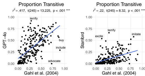
Figure 13: Evaluating the GPT-4o and Stanford Parsers’ estimates of transitivity (i.e., NP frame) rates by comparing them to Gahl et al.’s (2004) gold-standard dataset. Results showed significant correlations for both parsers, but GPT-4o (left) produced a better fit ( r^2 = .417 ) than the Stanford Parser (right; r^2 = .220 ).
