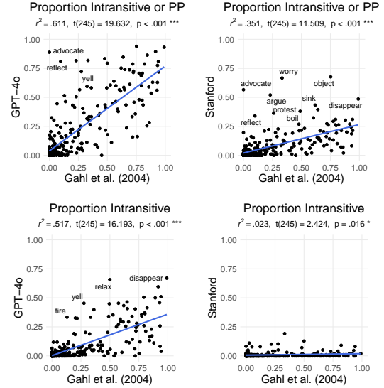
Figure 21: Evaluating the effect of including PP frames in intransitivity counts. For both the GPT-4o (left) and Stanford (right) parsers, including PPs (as Gahl et al. (2004) did) produced a better fit (top) to Gahl et al.’s estimates than excluding them (bottom), meaning that Gahl et al. lost meaningful information by collapsing these categories.
