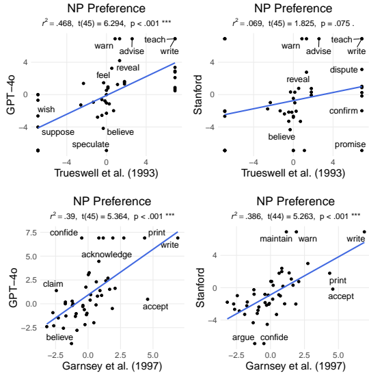
Figure 20: Evaluating GPT-4o (left column) and Stanford Parser (right) estimates of NP bias for NP/SC verbs. We compared our estimates to those from two prior studies: Trueswell et al. (1993; top row) and Garnsey et al. (1997; bottom). Both parsers significantly predicted the Garnsey et al. results, but only GPT-4o significantly predicted Trueswell et al.’s data.
