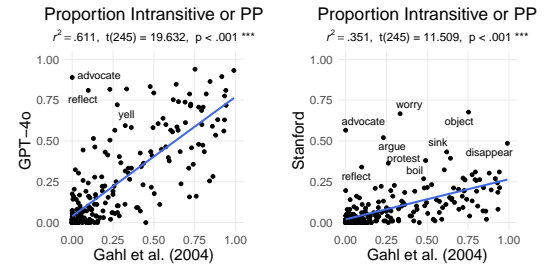
Figure 14: Comparing the GPT-4o and Stanford parsers’ intransitivity rates to Gahl et al. (2004) . To facilitate comparison, we followed Gahl et al. and counted prepositional phrase (PP) complements as intransitive for this analysis. GPT-4o (left) produced a better fit ( r^2 = .611 ) than the Stanford Parser (right; r^2 = .351 ).
