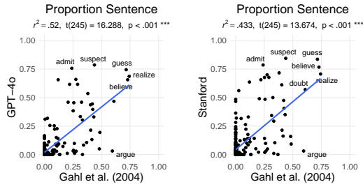
Figure 15: Comparing our estimates of sentential complement (SC; e.g., believe [that you can do it] SC ) frequencies per verb to Gahl et al. (2004). GPT-4o (left) accounted for more variance than the Stanford Parser (right).
