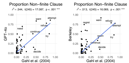
Figure 12: Comparing our estimates of nonfinite clausal complements (e.g., he refused to try ) frequencies per verb to Gahl et al. (2004). GPT-4o (left) accounted for more variance than the Berkeley Neural Parser (right).
