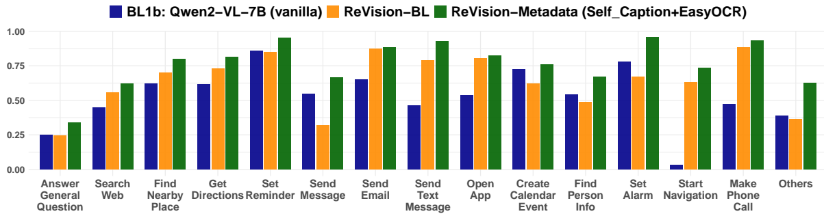
Figure 4: Class-wise F1 Scores for Intent Classification
