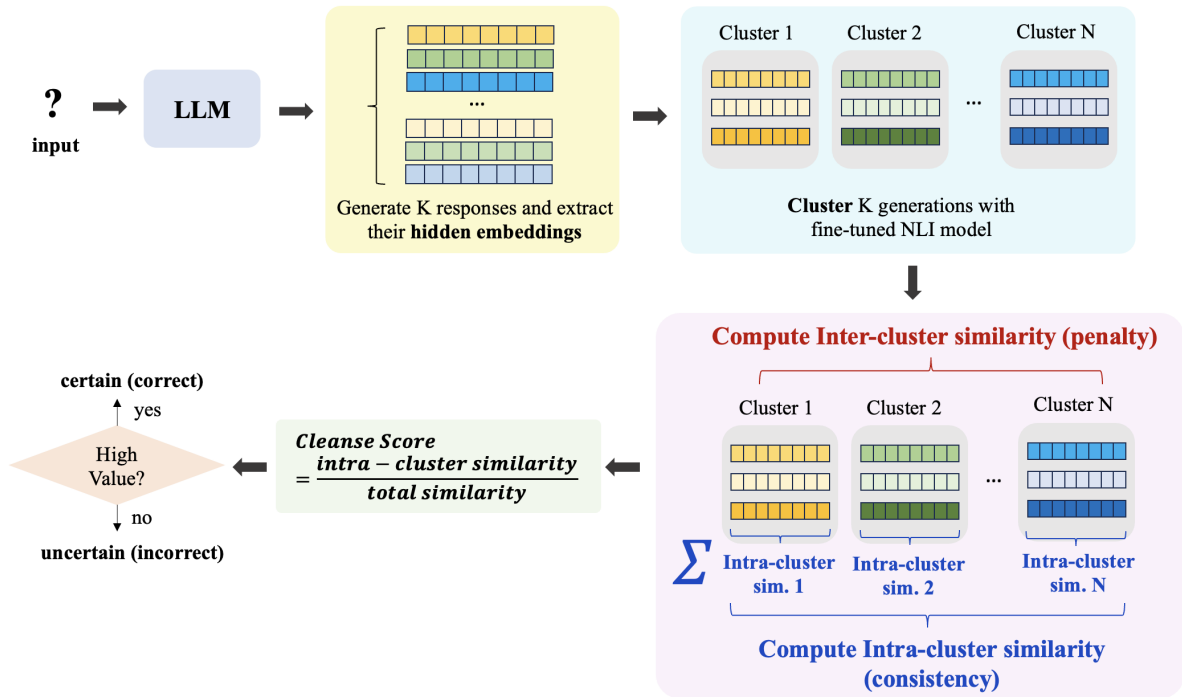
Figure 1: Illustration of Cleanse pipeline.
