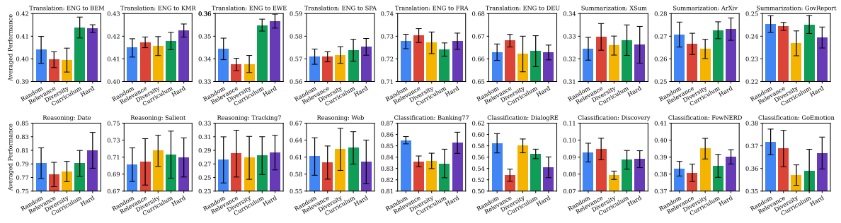
Figure 2: Results of various sample selection approaches on ICL of 64 examples with LCLMs, where we average the performance over all models: Gemini Pro, Gemini Flash, and Llama 3.1, across four different tasks with 18 datasets. Each bar represents the averaged performance, with the upper and lower limits indicating standard deviation. See Figure 9 for results on each model.
