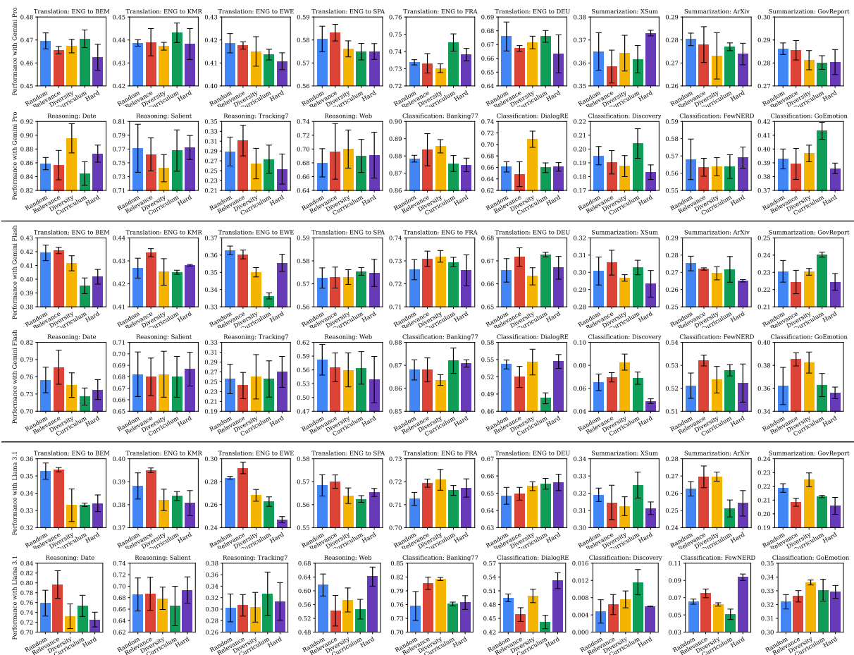
Figure 9: Detailed results of various sample selection approaches on ICL with LCLMs, such as Gemini Pro (Top), Gemini Flash (Middle), and Llama 3.1 (Bottom), across four different tasks (translation, summarization, reasoning, and extreme classification) with 18 datasets. Each bar represents the averaged performance, with the upper and lower limits indicating standard deviation.
