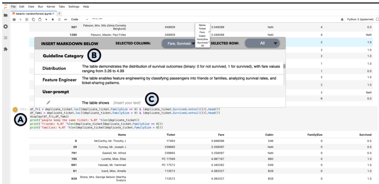
Figure 2: We implement a downstream application as a Jupyter Notebook plugin (A) to assist users in documentation writing for selected rows and columns from different guideline categories (B) and a user-prompt approach (C).
