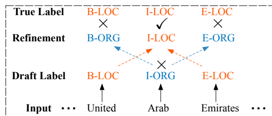
Figure 1: Schematic of label refinement framework (Cui and Zhang, 2019). The goal is refining the label of “Arab” using contextual labels and words, while the refinement of other correct labels may be negatively impacted by incorrect draft labels.
