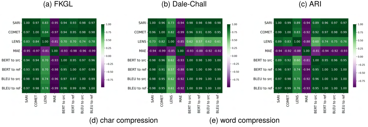
Figure 18: Pearson correlation heatmaps analyzing metric correlation, aggregated across all models. Dataset: SIMPA.
