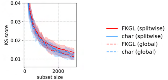
Figure 5: WIKILARGE. A comparison of split-based and split-agnostic sampling shows the latter yields lower divergence across both length and readability, with FKGL and N chars yielding similar results.
