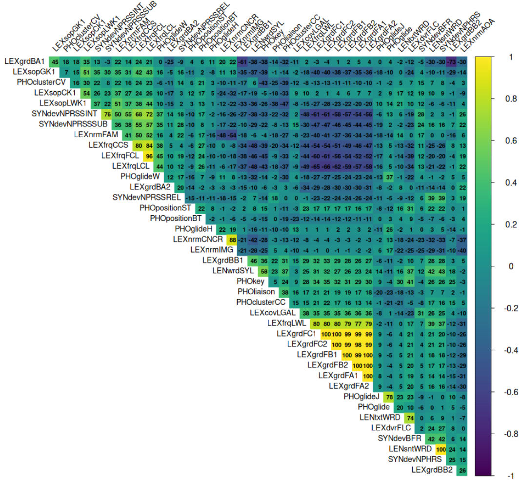
Figure 6: Correlation heatmap among the readability and phonemic features on the Alector texts
