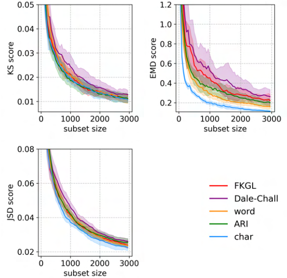
Figure 4: WIKILARGE. Global sampling with stratification by readability and length, measured in terms of KS, EMD and JSD. Stratification by N chars shows smallest divergence across all metrics.
