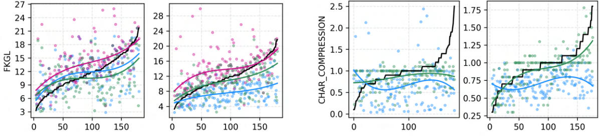
Figure 13: Dataset: WIKILARGE
