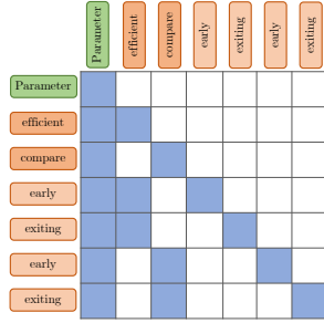
Figure 14: The attention mask for the tree draft is composed in such a way that child tokens can attend to all predecessors starting from the root, with the root being the correction issued by the main stream. In this illustration, “early” attends to “parameter” and “efficient” and itself, as “parameter - efficient - early” forms one path in the tree. “early” is also replicated to form another path, “parameter - compare - early”. This attention mask allows batching multiple paths and increases the acceptance rate as the number of candidates increases.
