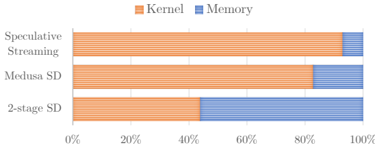
Figure 17: Kernel and Memory utilization comparison on Nvidia A100.
