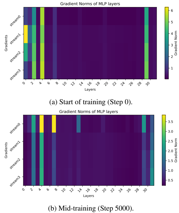
Figure 6: We visualize gradient norms across MLP layers due to speculative stream losses at the start of training and at step 5000. Early in training, speculative supervision injects strong gradients not only in later layers but also in early and mid-level MLP blocks, indicating that future-token predictions influence earlier computations via differentiable speculative paths. As training progresses, gradients become more structured and selective.
