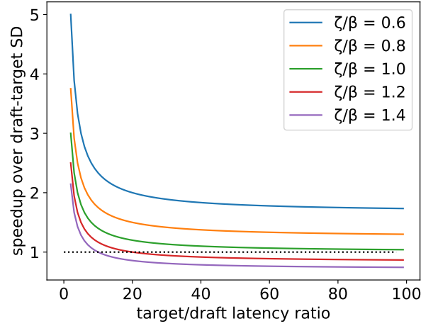
Figure 18: Speedup: Speculative Streaming speedups over draft model based speculative decoding for different \zeta/\beta and target/draft latency ratios, where \zeta denotes the number of advancements per verification step for draft model based speculative decoding while \beta denotes the same for Speculative Streaming.
