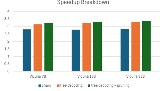
Figure 12: Ablation of effectiveness of Speculative Streaming components across Vicuna model scales. Chain denotes linear speculation via multi-stream attention as detailed in Section 2.1. Tree decoding enables parallel verification across batch trajectories as detailed in Section 2.2, while Tree pruning reduces redundant target verifications as detailed in Section 2.3. Together, these mechanisms compound to yield scalable speedup.
