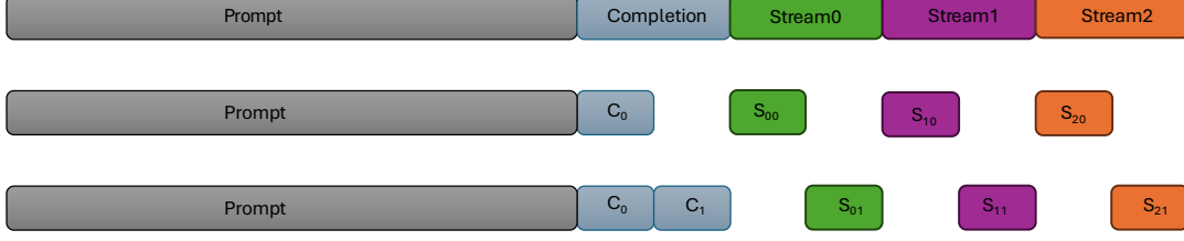
Figure 15: Streams corresponding to prompt are not required while training. Completion is divided into multiple segments and streams of each segment only attend to previous streams from same segment and main stream of previous segments. Uncolored portion indicates those tokens/streams are not required to be kept in memory.
