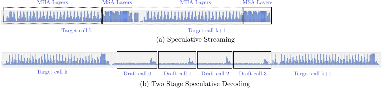
Figure 16: Kernel utilization timeline for speculative streaming and the standard draft-target speculative decoding. Draft-target approach runs speculation and verification in serial manner while it is parallelized in Speculative Streaming. Auto-regressive draft generation often has low GPU utilization leading to decreased overall kernel utilization while MSA layers in Speculative Streaming increase kernel utilization by generating a non-autoregressive draft and speeding up decoding significantly.
