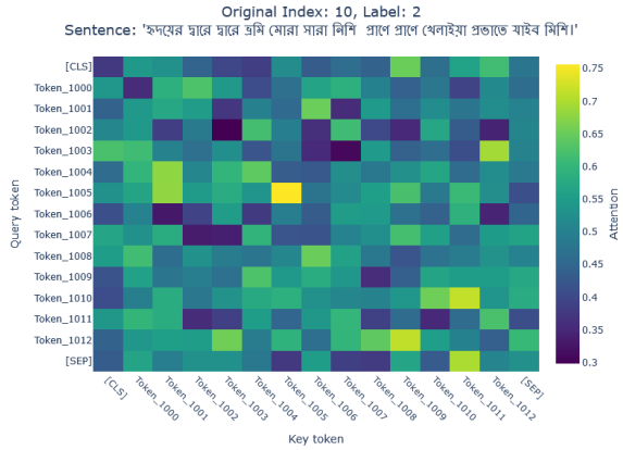
Figure 16: Attention heatmap generated by Llama for a misclassified FoS identification sentence with multiple FoS labels.
