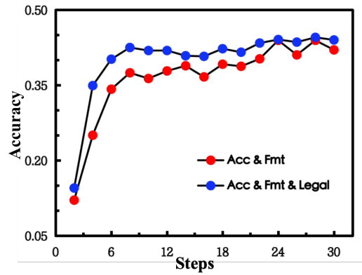
Figure 4: Comparison of convergence behavior of Unilaw-R1-SFT under different combinations of reinforcement learning reward functions on the Unilaw-R1-Eval benchmark.
