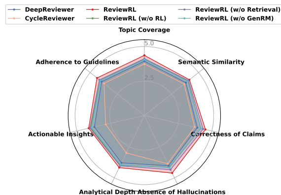
Figure 1: Evaluation results of ReviewRL under the criteria of ReviewEval (Kirtani et al., 2025)
