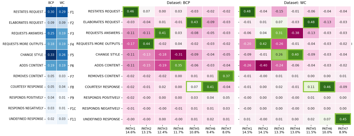
Figure 3: (a) The fraction of sessions which contain a follow-up type. (b) The correlation between follow-up types and principal components (PC) inferred by PCA. Each PC represents a PATH. Large positive values (green boxes) indicate stronger correlations. The percentages (bottom) depict the variance explained by each PATH.
