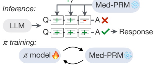
Figure 1: Overview of the MED-PRM. (1) An LLM generates reasoning traces for medical questions, and relevant documents are retrieved from external corpora. (2) A large LLM assigns stepwise labels (+/-) for each reasoning step. (3) These labeled traces are used to train the Med-PRM reward model. (4) Med-PRM reward model is used for inference-time evaluation or further train the policy model.
