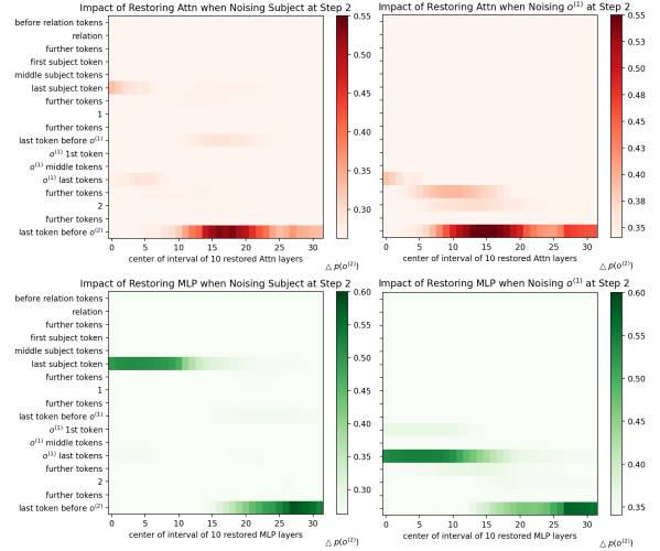
Figure 3: The impact of attention and MLPs’ activations on LMs’ predictions when intervening on the subject (left) and previous answer tokens (right) at step 2. The probability differences all peak around or above 0.55, reflecting the importance of both the subject and previous answer tokens. See Appx. §D for figures of other answer steps, which have similar patterns.
