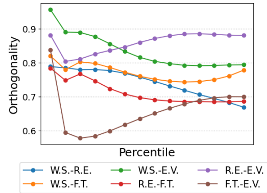
Figure 10: Trends of orthogonality functions with the change in percentile of different pairs of raters.
