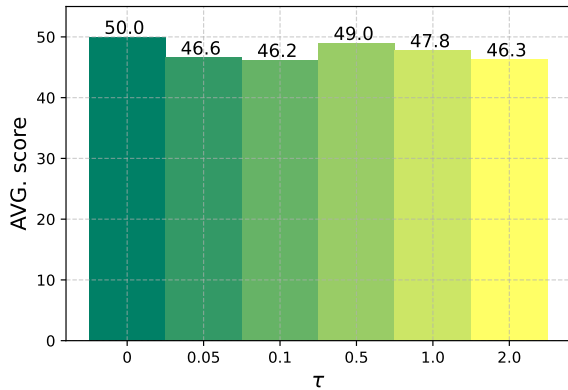
Figure 12: The impact of the sample temperature coefficient on model performance. \tau is the temperature coefficient, and when \tau = 0 , it refers to top-K selection.
