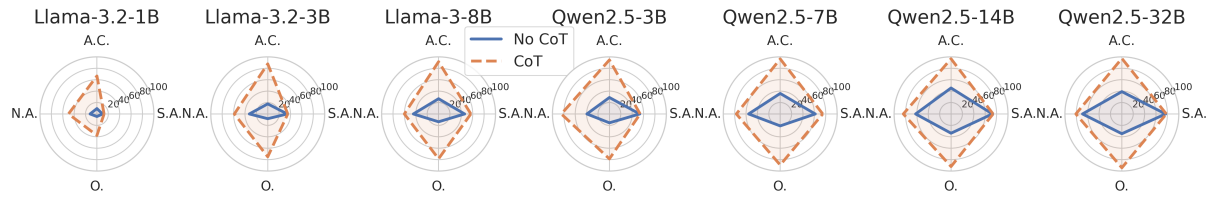
Figure 10: Model zero-shot with and without CoT performance on GSM8K. A.C.: Arithmetic Computation; N.A.: Numerical Abstraction; O.: Original; S.A.: Symbolic Abstraction.
