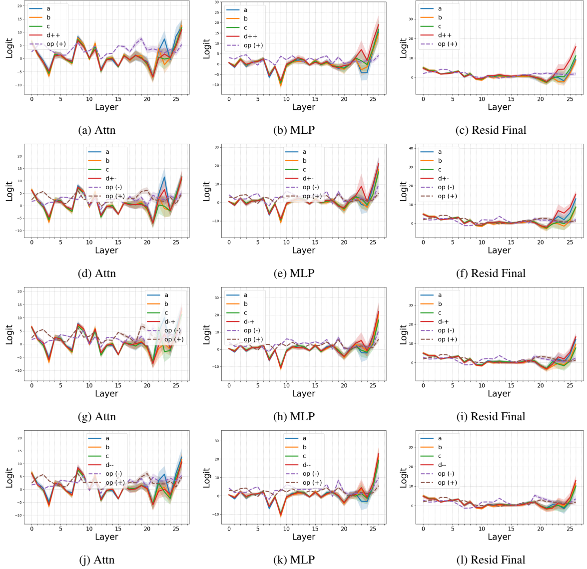
Figure 27: Visualizations of internal computations at last token position in Qwen 2.5 7B for two-operation math word problems. First row: for a + b + c . Second row: for a + b - c . Third row: for a - b + c . Fourth row: for a - b - c .
