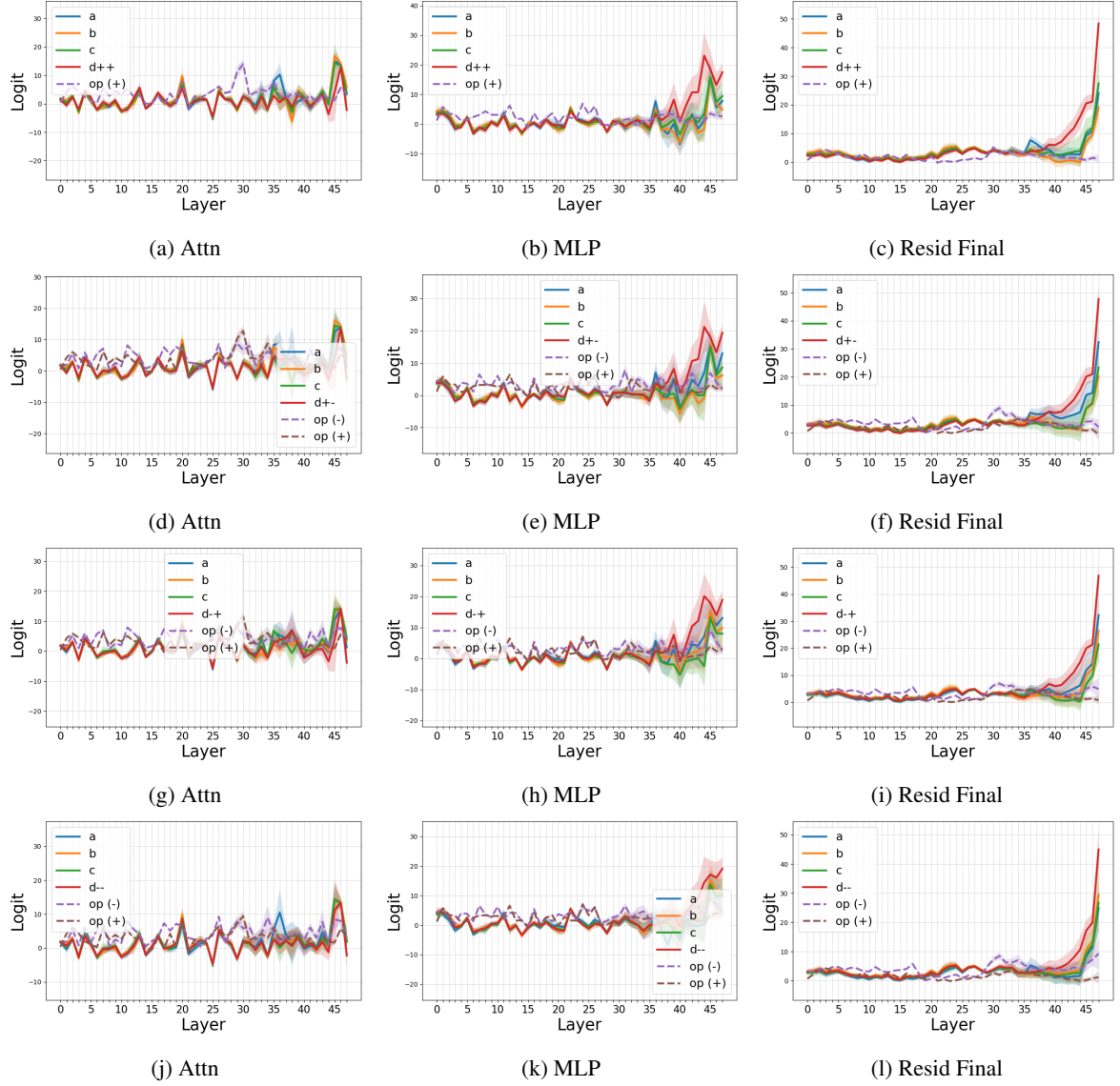
Figure 28: Visualizations of internal computations at last token position in Qwen 2.5 14B for two-operation math word problems. First row: for a + b + c . Second row: for a + b - c . Third row: for a - b + c . Fourth row: for a - b - c .
